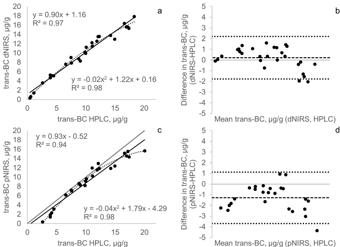
Fig 3. Scatterplot and Bland Altman comparison between trans-BC measured by HPLC versus dNIRS (a-b) and pNIRS (c-d). The black lines indicate linear regression lines and the dotted lines indicate quadratic regression lines. Gray lines represent the line of identity. The square dotted lines represent the bias and the round dotted lines indicate the 95% confidence interval.
